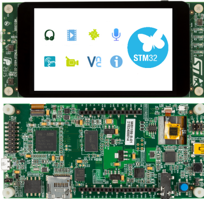
Board top and bottom views. Pictures are not contractual.
