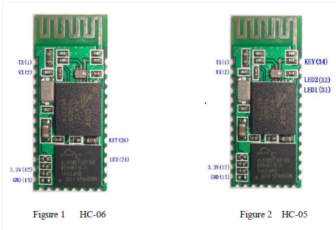
— HC-06 and HC-05 (Source Wavesen Data Sheet)
