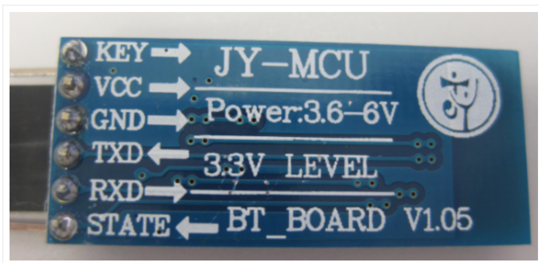
— JY-MCU BT_BOARD V1.05 Bottom Side
