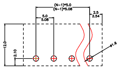
PCB LAYOUT(RECOMMENDED) (TOP VIEW TOL. :±0.05)
