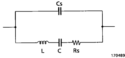
Figure 3.3.2 (b) Oscillator Equivalent Circuit
