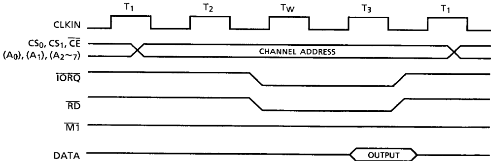
Figure 3.4.5 Read Timing
