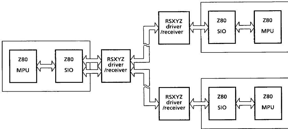
Figure 3.5.14 (a) Example of Data Communication Between Processors
