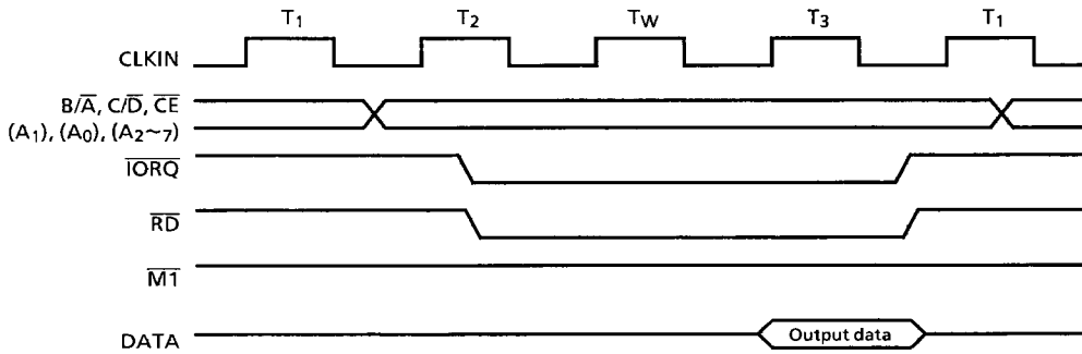
Figure 3.5.9 Read Timing
