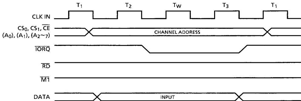
Figure 3.4.4 Write Timing
