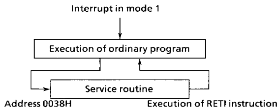
Figure 3.2.7 Interrupt Processing in Mode 1
