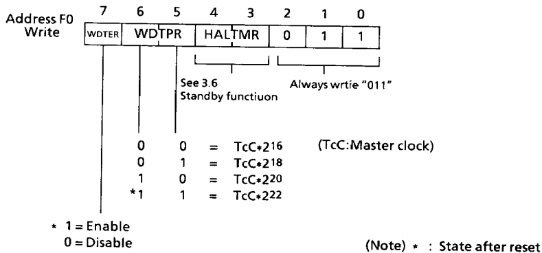
Figure 3.7.2 Enabling Watching Timer
