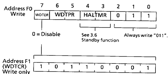
Figure 3.7.3 Disabling Watchdog Timer
