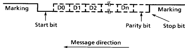
Figure 3.5.4 Data Format of Asynchronous Mode
