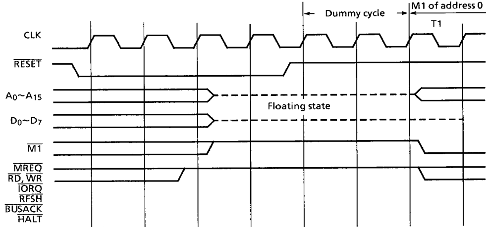
Figure 3.2.21 Reset Timing
