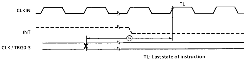
Figure 4.4.15 CTC Interrupt Occurrence Timing
