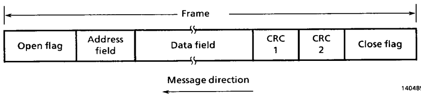
Figure 3.5.6 Data Format in SDLC Mode
