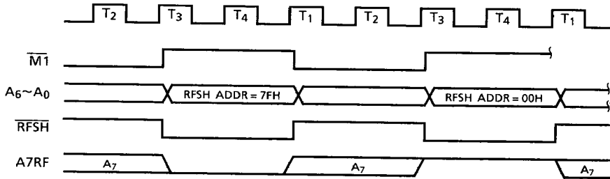
Figure 3.2.11 Refresh Timing
