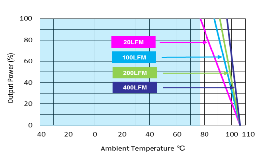
MJWI15-24S033, MJWI15-48S033 Derating Curve with Heatsink
