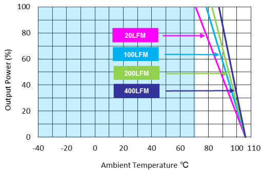
MJWI15-24S15, MJWI15-24D12, MJWI15-24D15 MJWI15-48S12, MJWI15-48S15, MJWI15-48D15 Derating Curve without Heatsink
