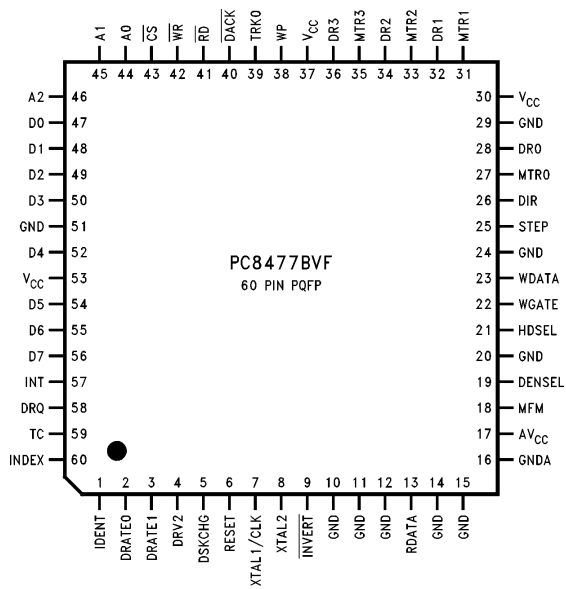
Plastic Quad Flat Package (VF) Order Number PC8477BVF-1 See NS Package Number VF60A
