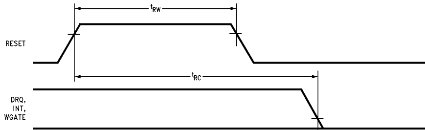
FIGURE 6-5. Reset Timing
