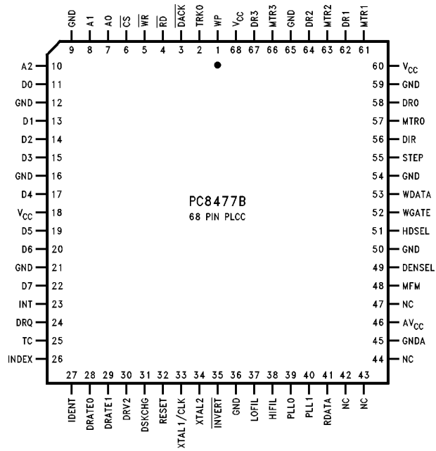
Plastic Chip Carrier (V) Order Number PC8477BV-1 See NS Package Number V68A
