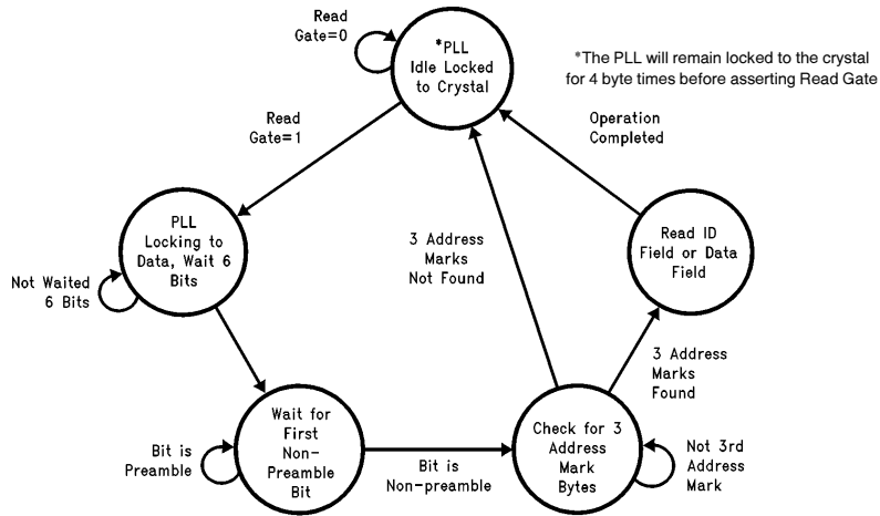
FIGURE 5-2. Read Data Algorithm—State Machine
