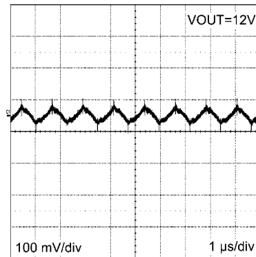
Output Ripple
