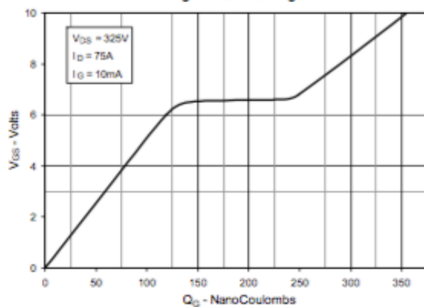
Fig. 11. Gate Charge
