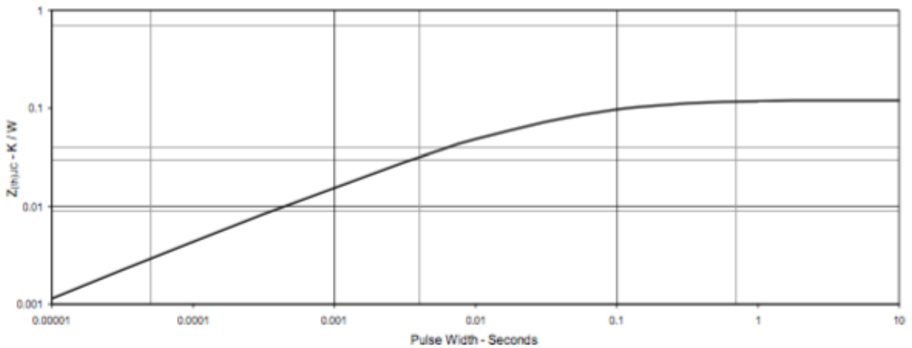
Fig. 15. Maximum Transient Thermal Impedance
