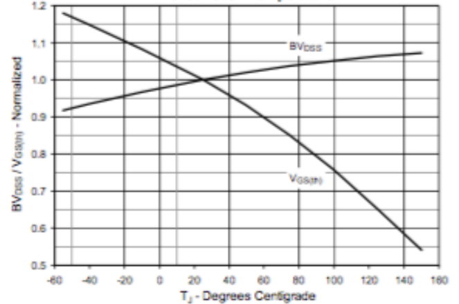
Fig. 6. Normalized Breakdown & Threshold Voltages vs. Junction Temperature
