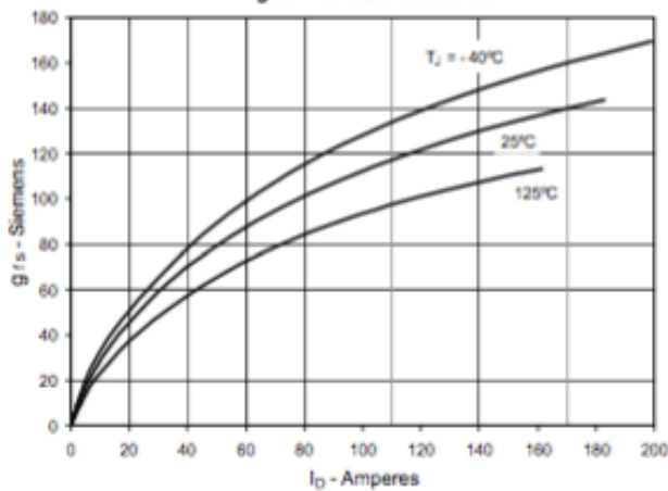
Fig. 9. Transconductance
