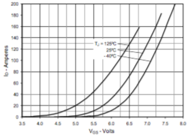
Fig. 8. Input Admittance
