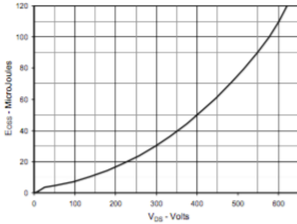
Fig. 13. Output Capacitance Stored Energy
