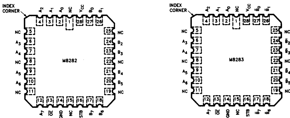
Figure 2. Pin Configurations
