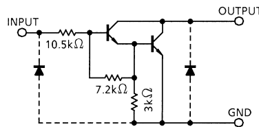
TD62104P / F
