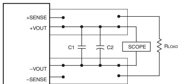
C1 = 0.47µF CERAMIC C2 = NA LOAD 2-3 INCHES (51-76mm) FROM MODULE
