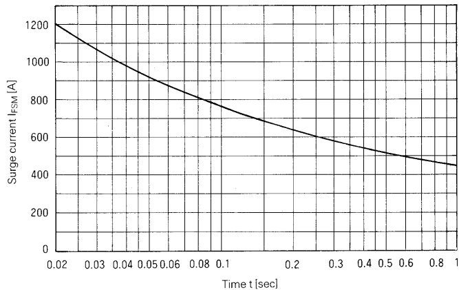
Surge Current
