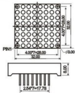
CPM12088
