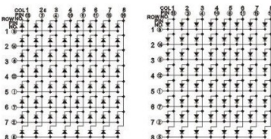
PCB:M19088C/D
