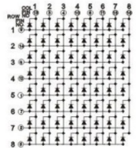
PCB:M12088A/B
