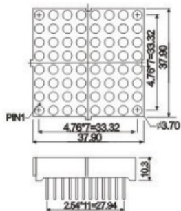
CPM15088
