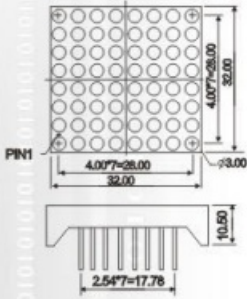
CPM12188
