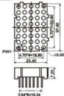
CPM14058
