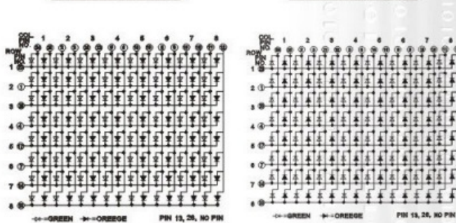
PCB:M19088E/FEG
