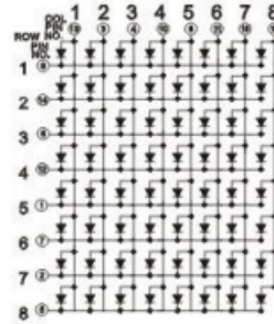
PCB:M12088A/B
