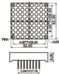
CPM12088
