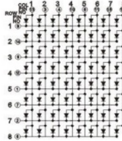
PCB:M12088A/B
