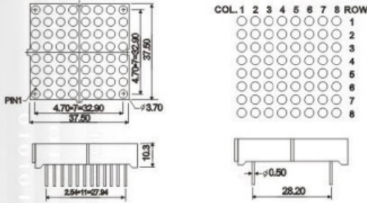
CPM15288
