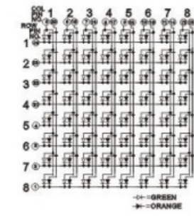
PCB:M15088A/BEG
