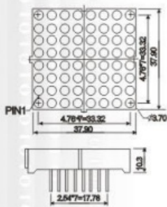
CPM15088
