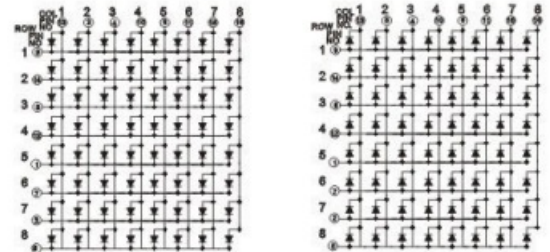
PCB:M15288A/B
