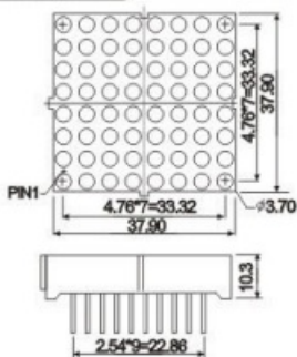
CPM15088
