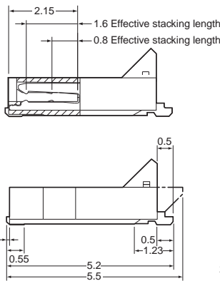
Cross-section diagram: X-X
