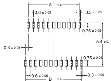
PCB Dimensions (TOP VIEW)
