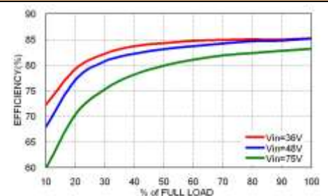
MOP06-48S05WA Efficiency vs. Output Load
