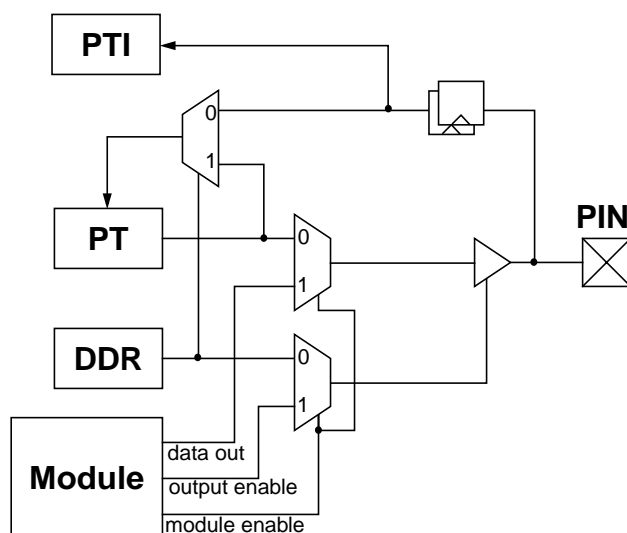
Figure 22-76. Illustration of I/O Pin Functionality
