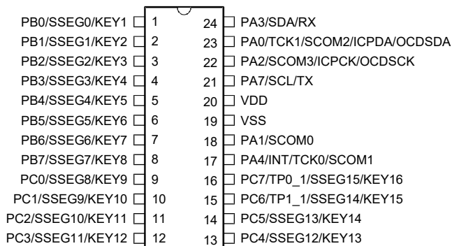
BS82C16A-3/BS82CV16A-3 24 SOP-A
