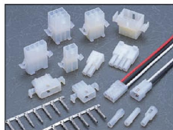
A00103 Series A10103 Series \phi 1.58mm Page: 102
