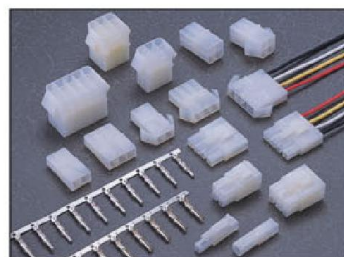
A00226 Series A10226 Series \phi 2.00mm Page: 109
