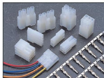
A00228 Series A10228 Series \phi 2.36mm Page: 117
