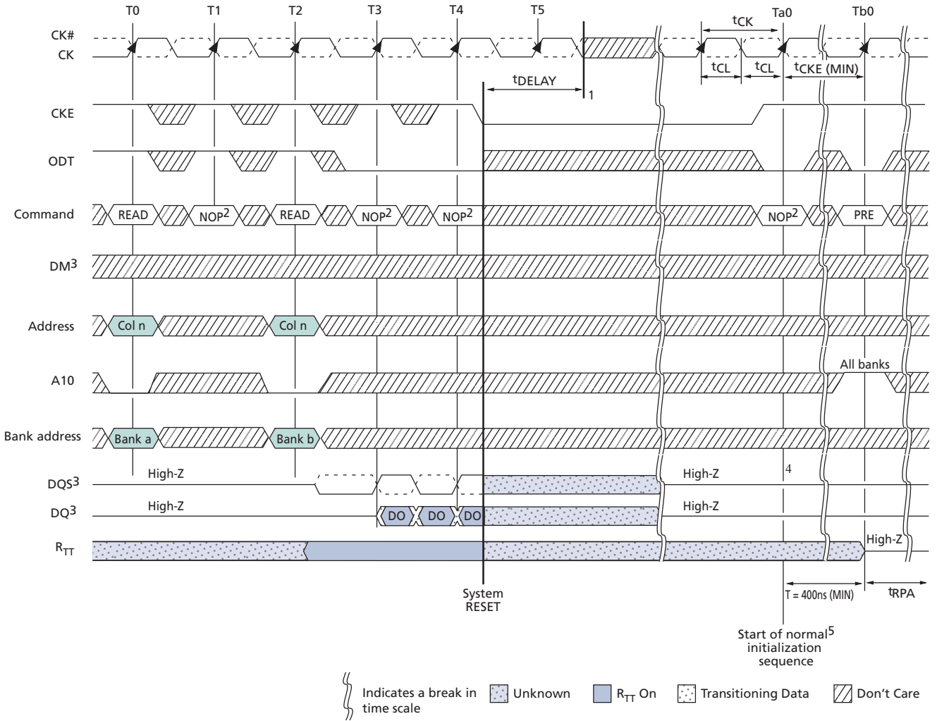
Figure 80: RESET Function
