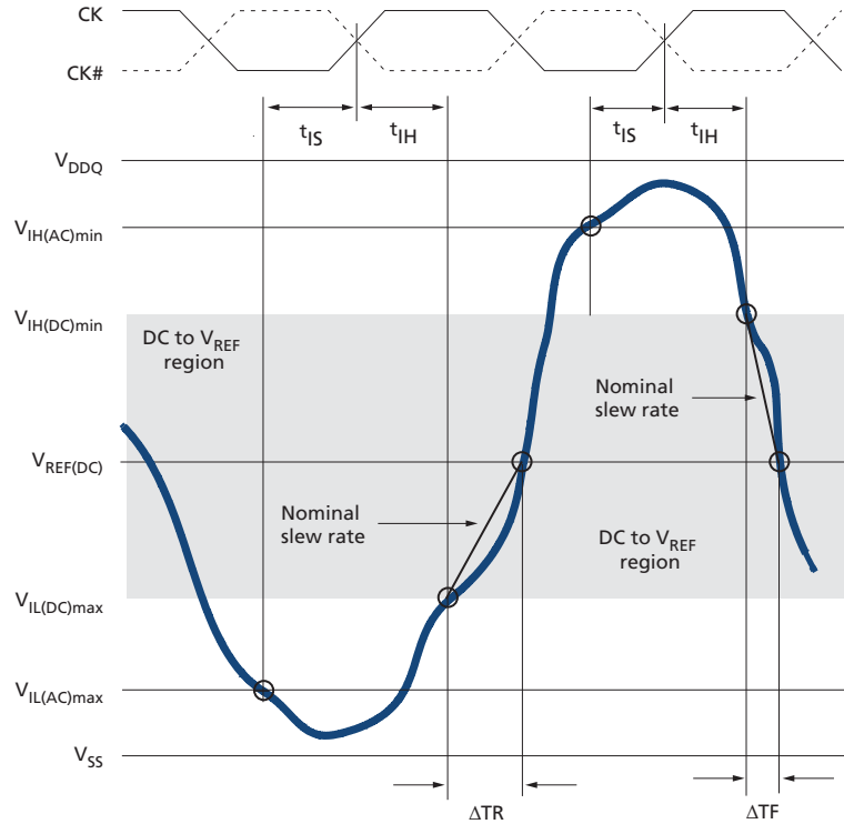
Figure 26: Nominal Slew Rate for t_{IH}
