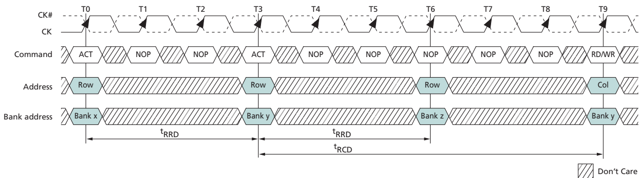
Figure 44: Example: Meeting t_{RRD} (MIN) and t_{RCD} (MIN)
