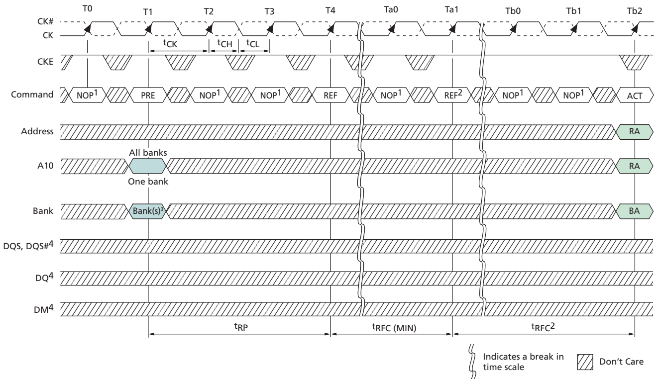
Figure 68: Refresh Mode
