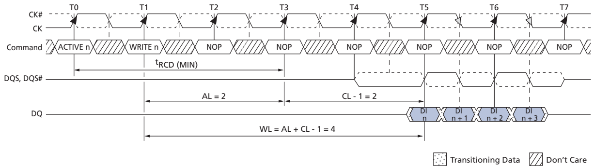
Figure 40: WRITE Latency
