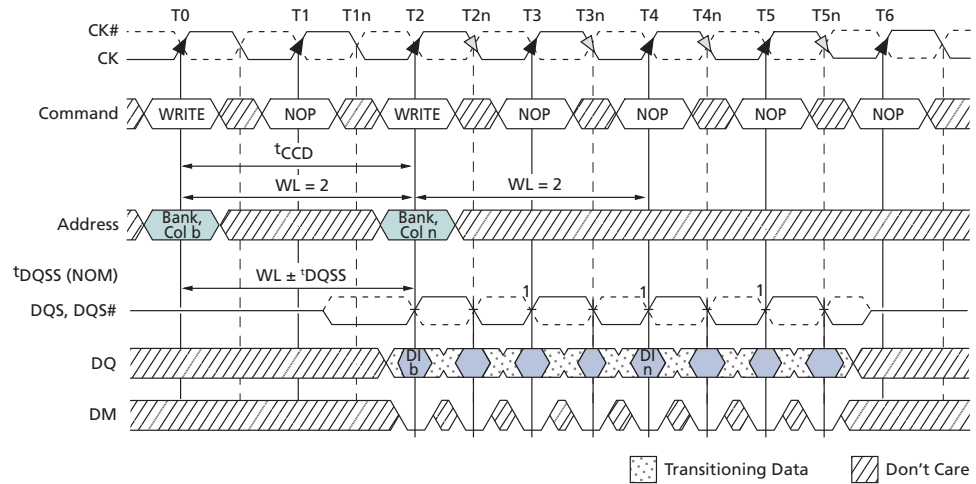
Figure 59: Consecutive WRITE-to-WRITE
