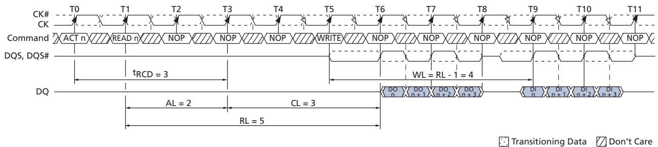
Figure 50: READ-to-WRITE
