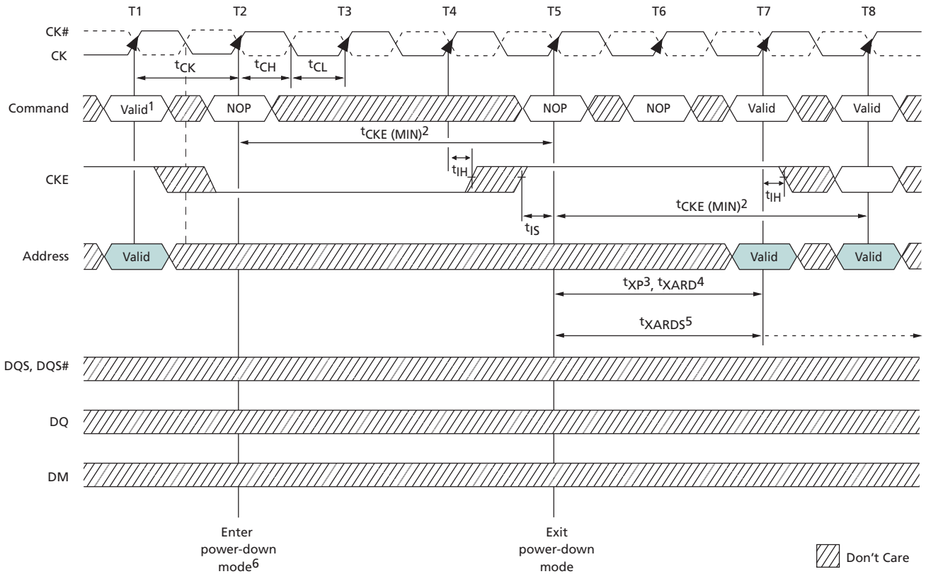
Figure 70: Power-Down
