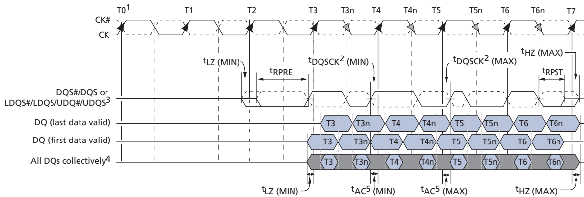
Figure 57: Data Output Timing – t_{AC} and t_{DQSK}
