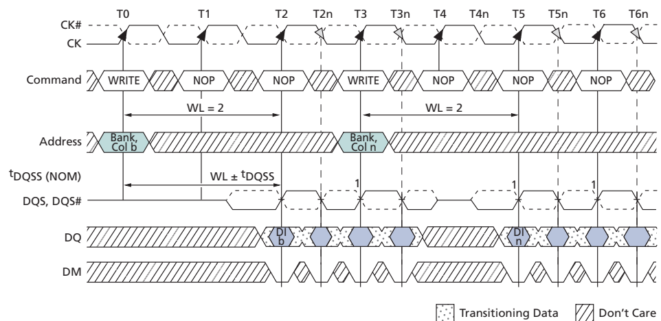
Figure 60: Nonconsecutive WRITE-to-WRITE
