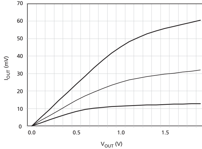
Figure 19: Reduced Strength Pull-Down Characteristics
