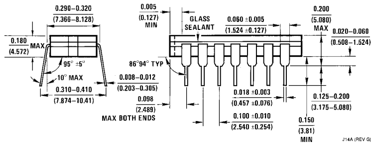
14-Lead Ceramic Dual-In-Line Package (J) Order Number 5410DMQB or DM5410J NS Package Number J14A
