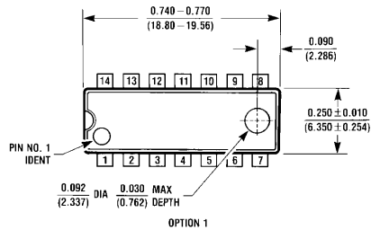
14-Lead Ceramic Dual-In-Line Package (J) Order Number 5410DMQB or DM5410J NS Package Number J14A
