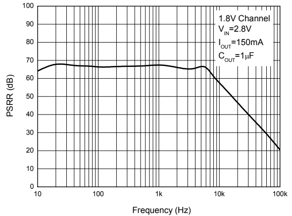
Figure 43. PSRR vs. Frequency
