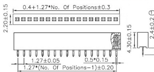
[ 1.27mm Female Header , 1 Row, Straight Type , 1*40 Poles ]
