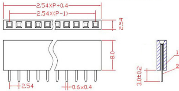
[ 2.00mm Female Header , 1 Row, Straight Type , 1*40 Poles ]
