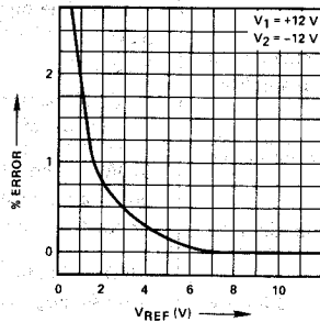
Ratio Operation (V IN /V REF = Constant)
