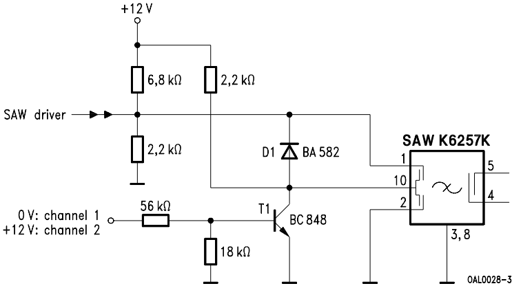
Figure 16 Switching network for a multistandard video filter
