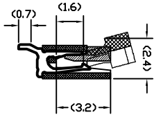
CFP-0520XS-WT SECTION A-A
