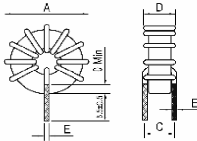
Figure 1 (standard type)
