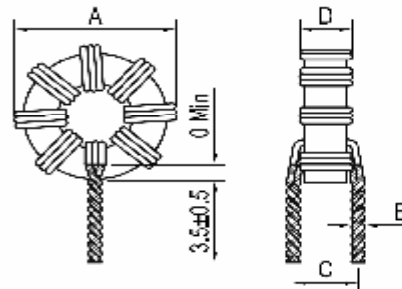
Figure 2 (multiwire type)
