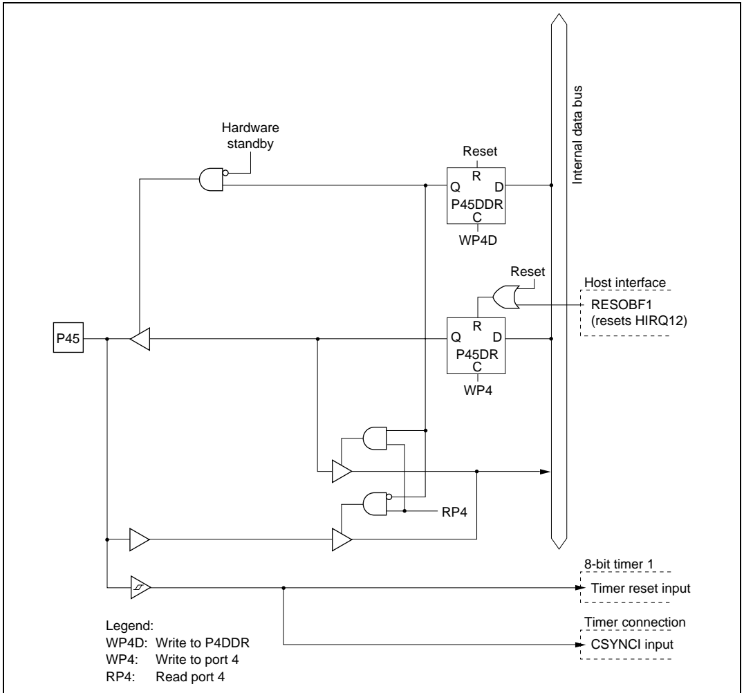
Figure C.11 Port 4 Block Diagram (Pin P45)
