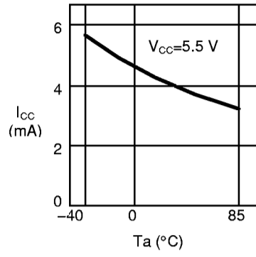
1.1 Operating current consumption I_{CC} – Ambient temperature T_a
