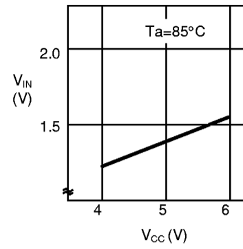
1.11 Input voltage V_{IN} – Power supply voltage V_{CC} S-24S Series : STORE and RECALL
