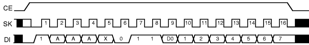
Figure 11 Write mode timing(S-24H30, S-24S30)
