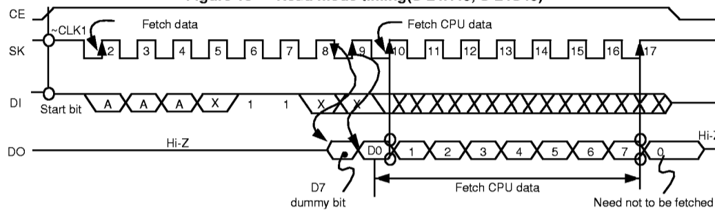
Figure 14 Read mode timing(S-24H30, S-24S30)
