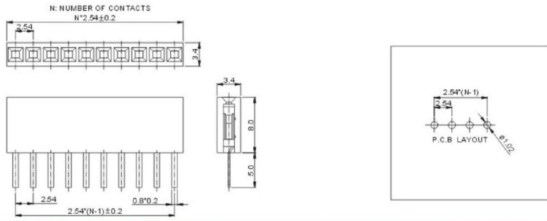
drawing of CE single row 2.54mm female header
