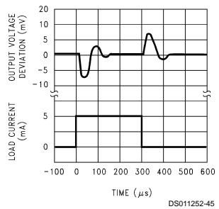
Load Transient Response ( V_{stby} )
