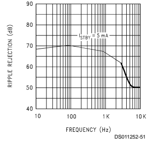
Ripple Rejection ( V_{STBY} )
