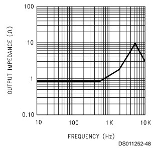
Output Impedance ( V_{stby} )
