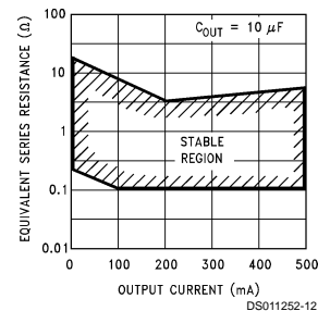
Output Capacitor ESR (Main Output, Pin 11)
