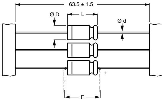
Form BR: Taped on reel Form BA: Taped in box (ammopack) Case Ø D x L = 4.5 mm x 10 mm to 8 mm x 11 mm
