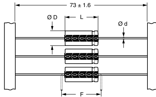
Form BR: Taped on reel Case Ø D x L = 6.5 mm x 18 mm to 15 mm x 30 mm Form BA: Taped in box (ammopack) Case Ø D x L = 6.5 mm x 18 mm to 10 mm x 25 mm
