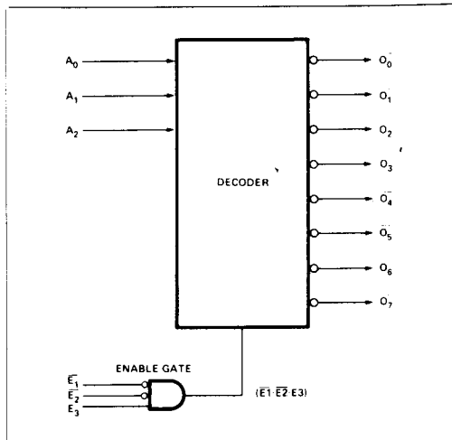
Figure 3. Enable Gate
