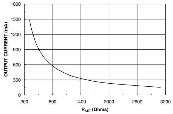
Figure 10. Current Limit vs. Rset
