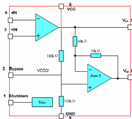
The block diagram of 8002
