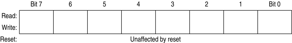
Figure 8-2. Accumulator (A)
