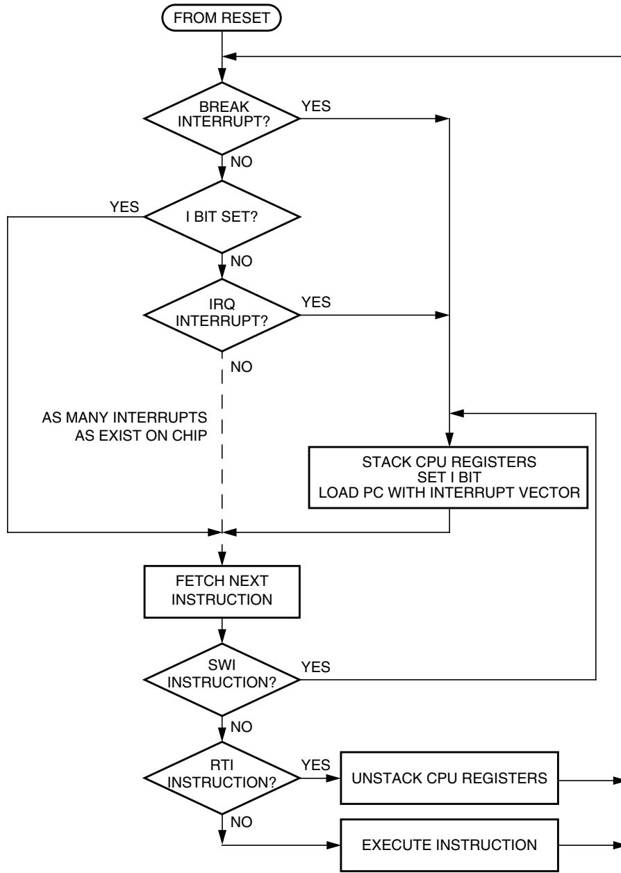
Figure 14-10. Interrupt Processing
