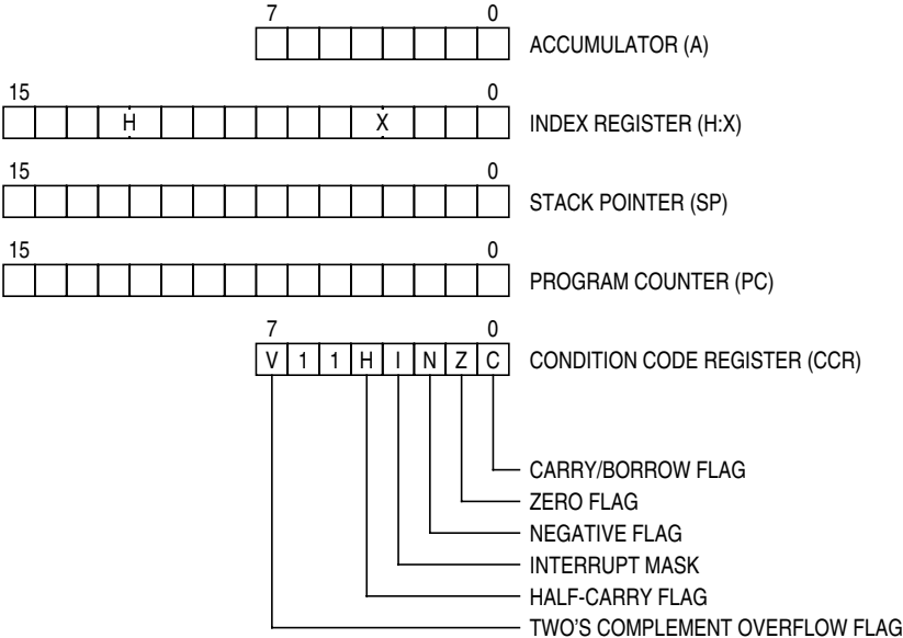
Figure 8-1. CPU Registers
