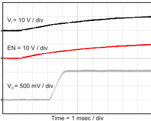
Figure 42. TPS563209 Start Up Relative to V 1
