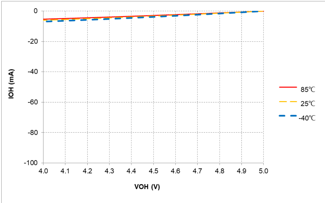
Figure 17-5 IOH vs. VOH @L0 = -3mA , VDD = 5V
