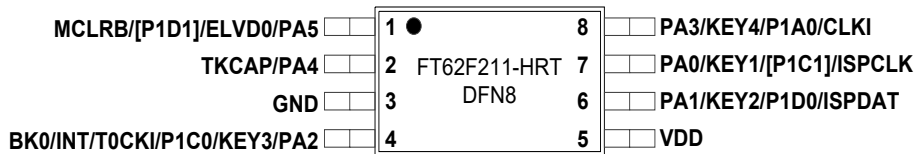
Figure 1-5 DFN8 3
