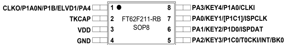
Figure 1-4 SOP8
