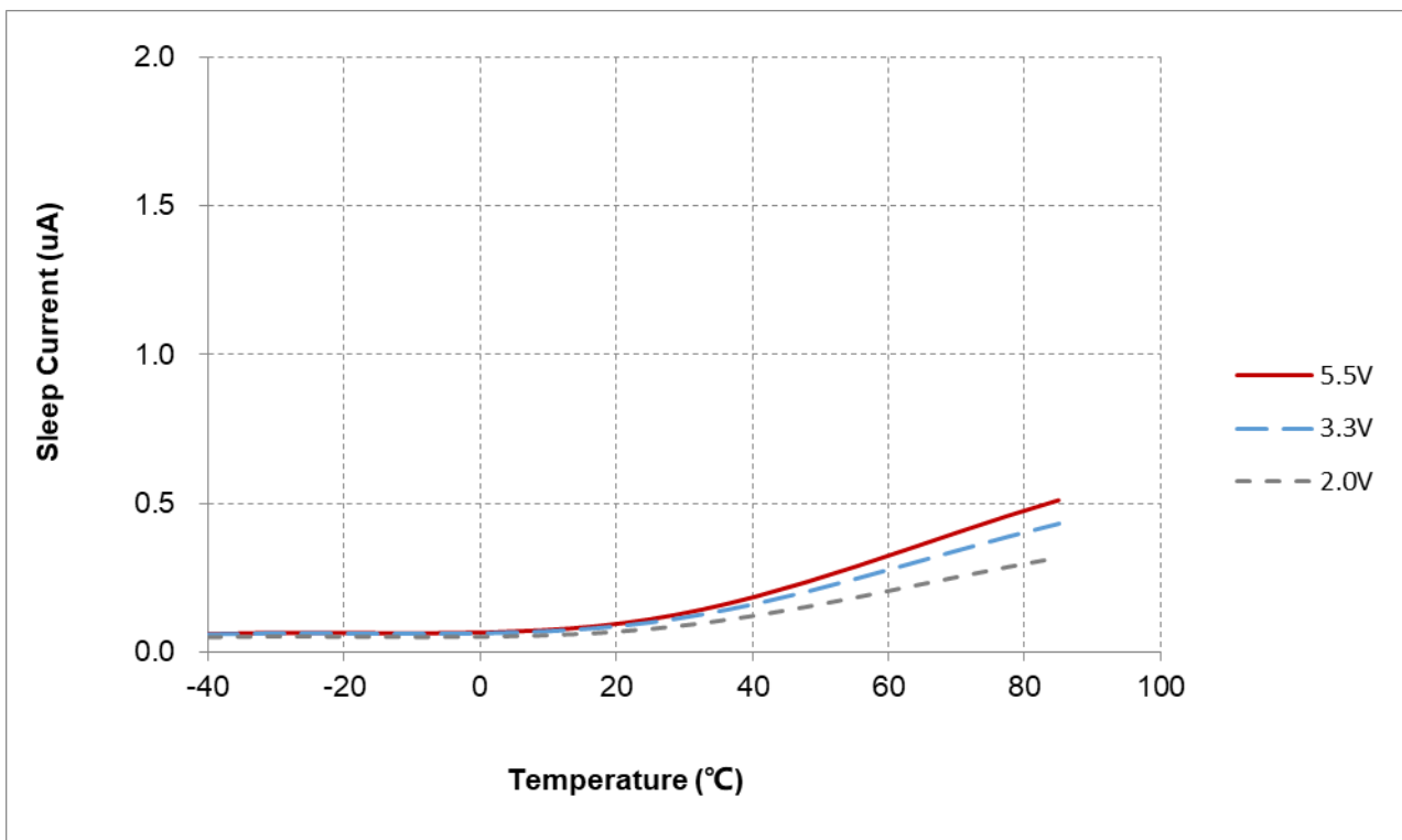
Figure 17-4 Sleep Current (I SB ) vs. Temperature
