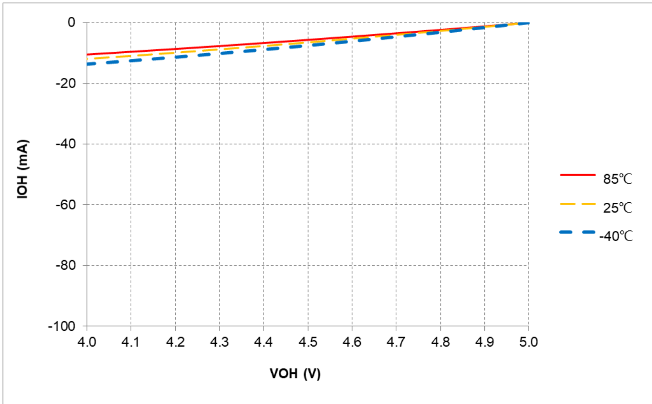
Figure 17-6 IOH vs. VOH @L1 = -6mA , VDD = 5V
