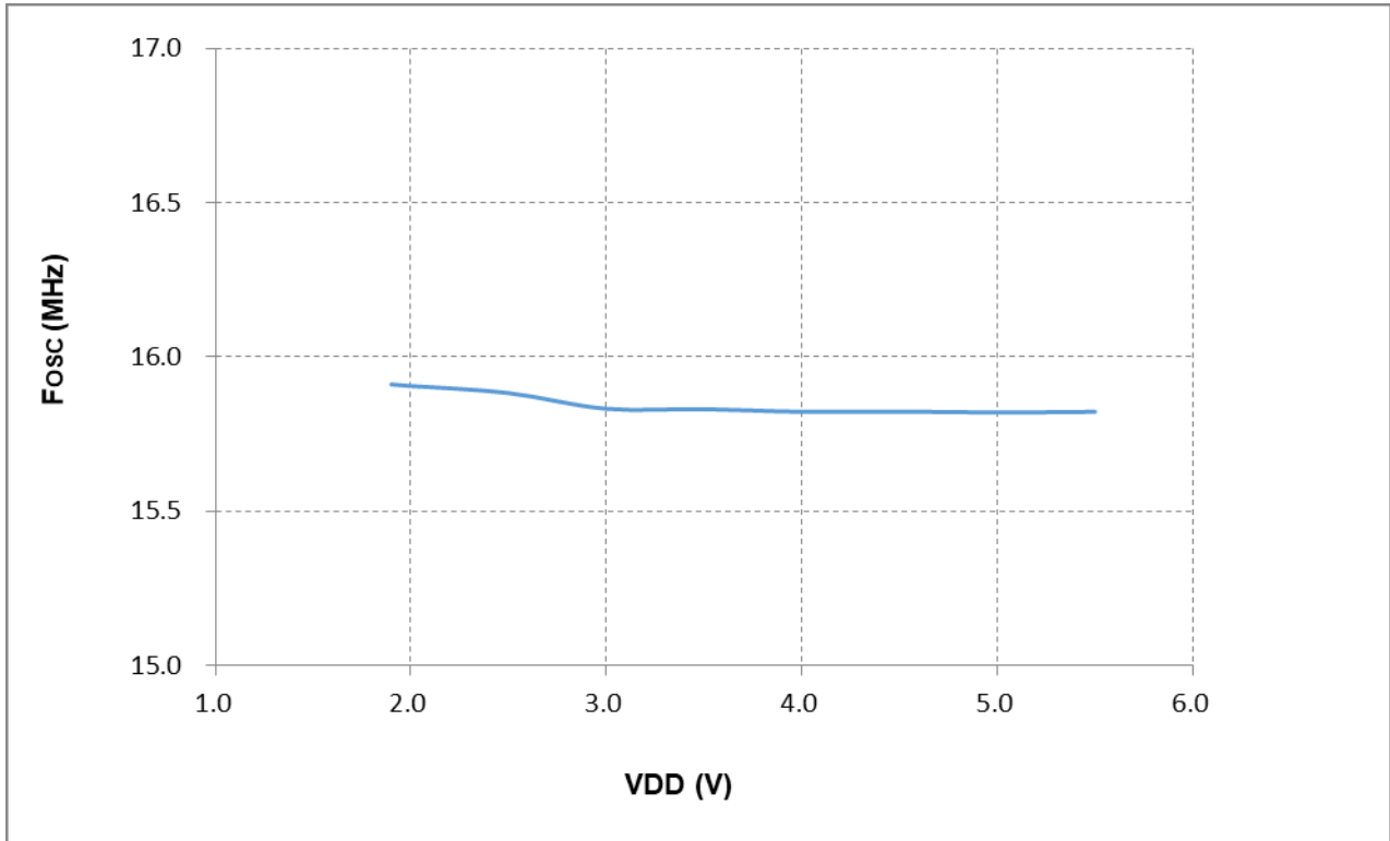
Figure 17-1 HIRC vs. V_{DD} ( T_A = 25^\circ\text{C} )
