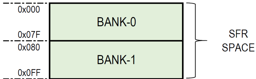
Figure 15-2 Indirect addressing
