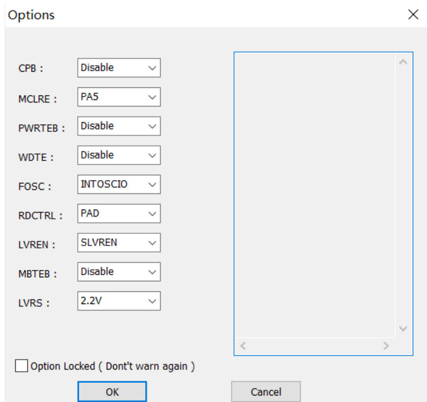
Figure 15-1 Boot Selectables in the IDE
