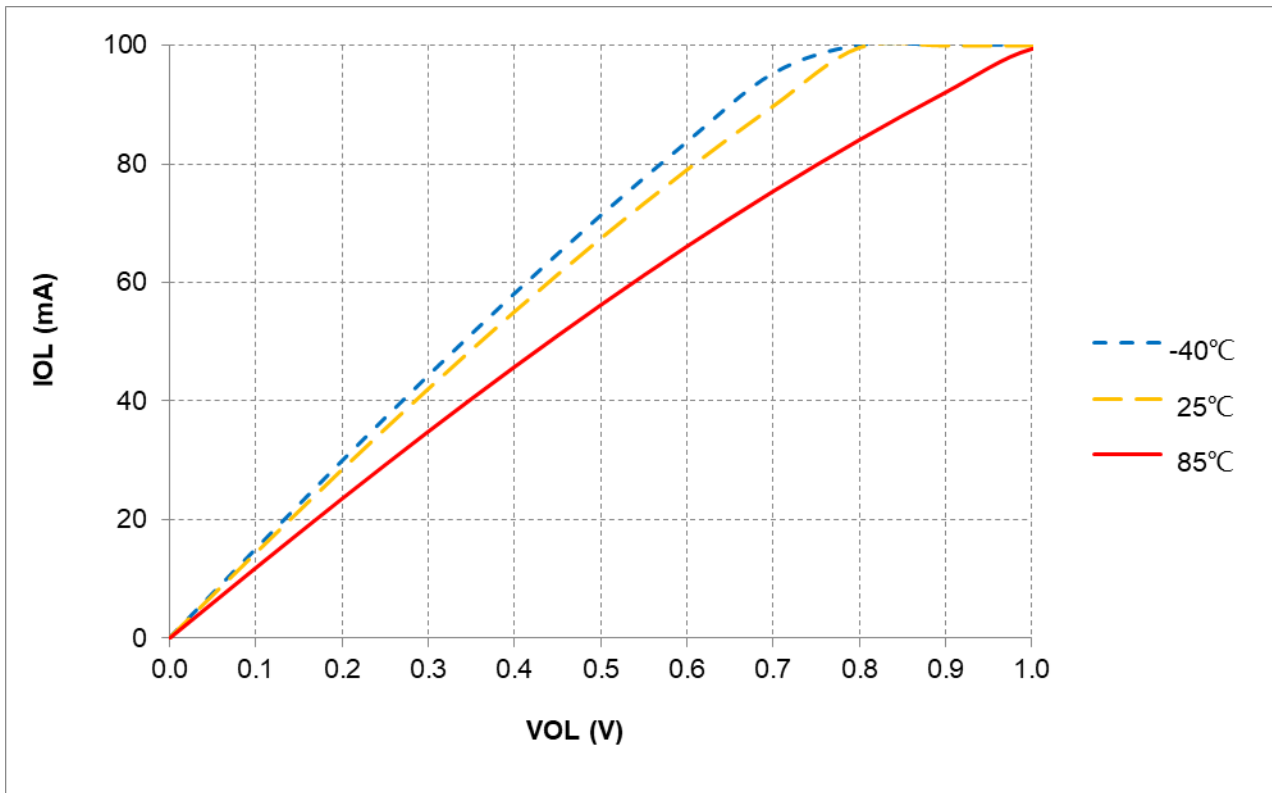
Figure 17-10 IOL vs. VOL @L1 = 67mA , VDD = 5V
