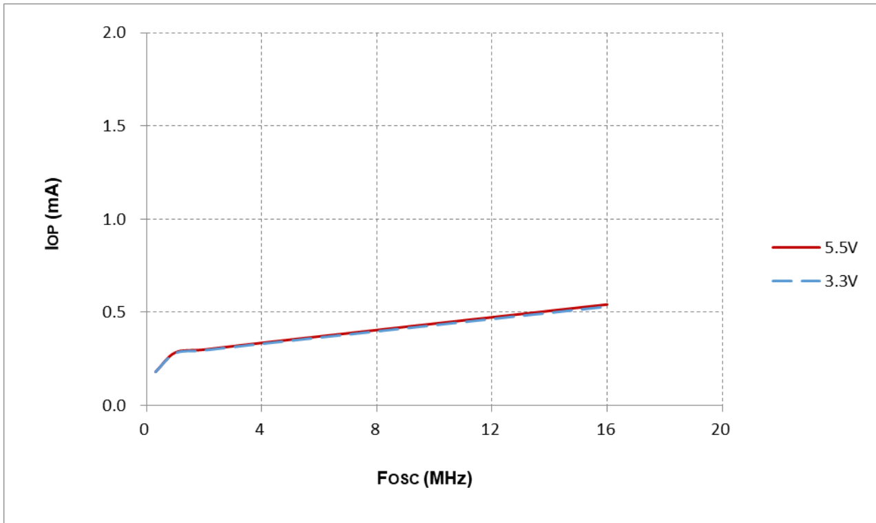
Figure 17-3 I DD vs. Frequency (4T, T A = 25°C)
