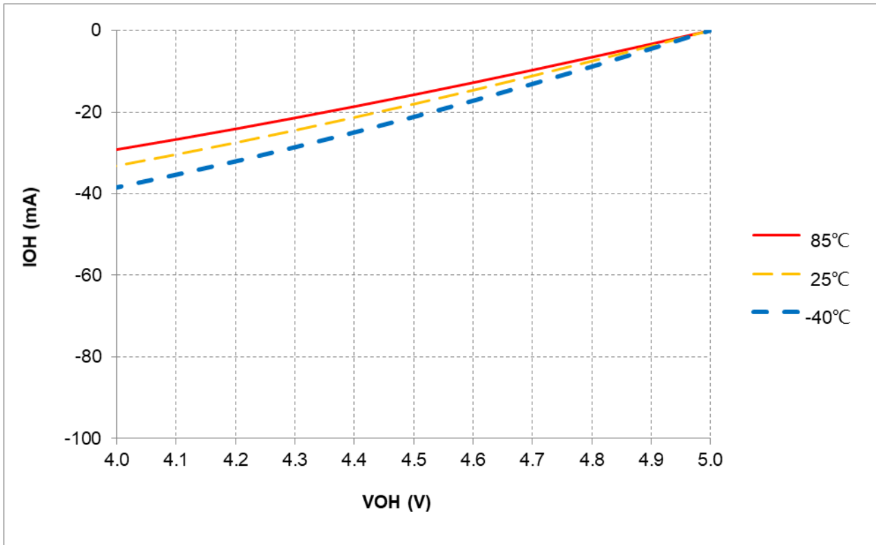
Figure 17-7 IOH vs. VOH @L2 = -18mA , VDD = 5V
