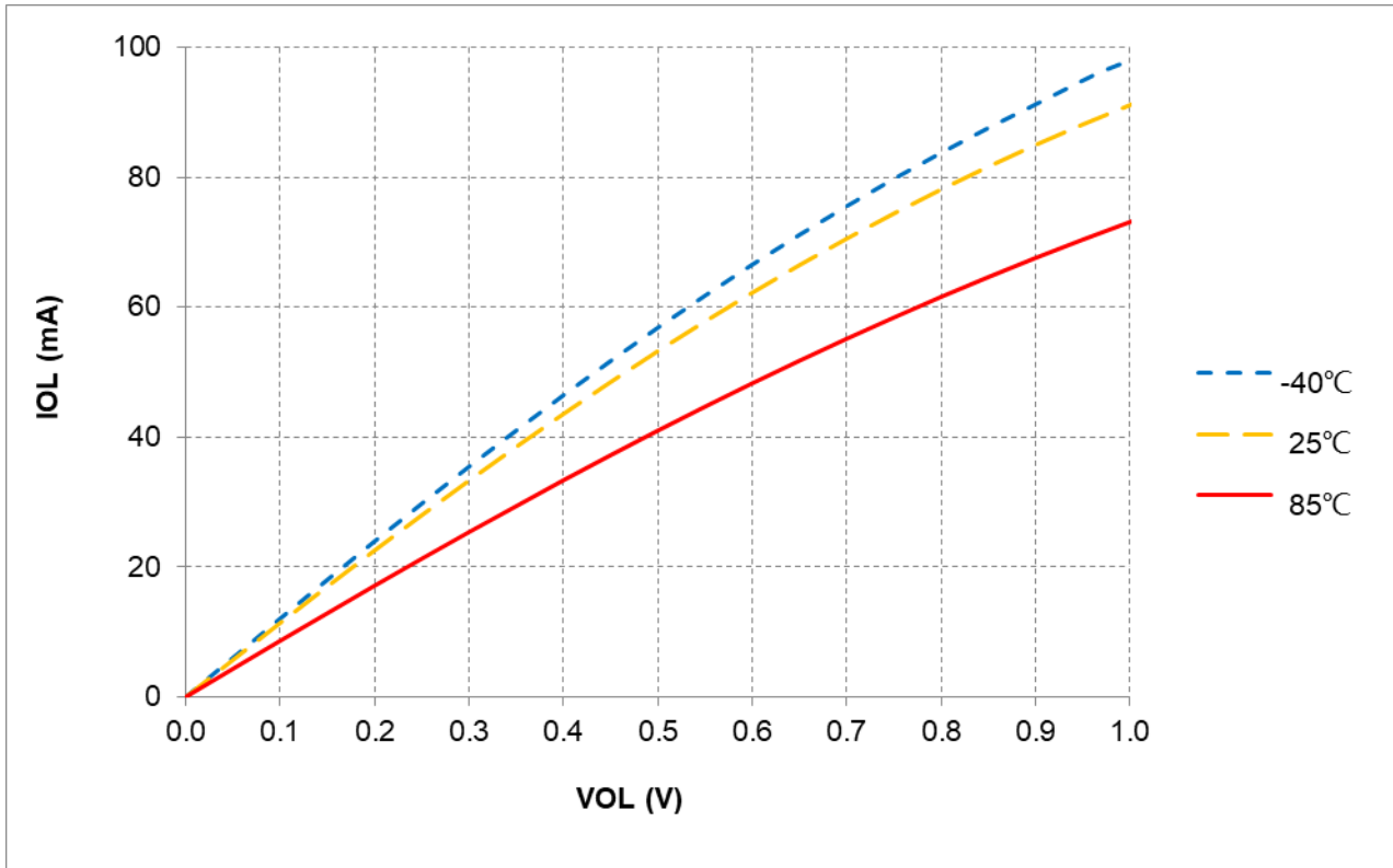
Figure 17-9 IOL vs. VOL @L0 = 53mA , VDD = 5V
