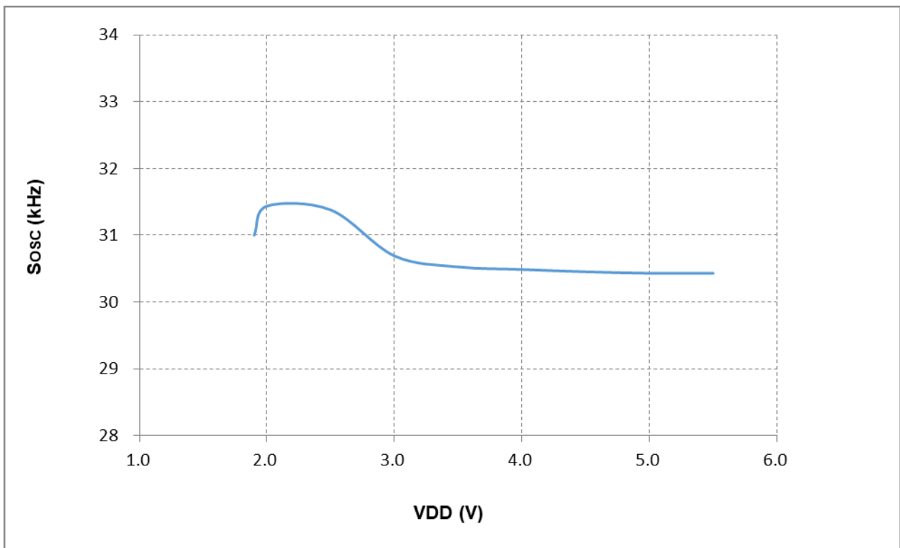
Figure 17-2 LIRC vs. V_{DD} ( T_A = 25^\circ\text{C} )
