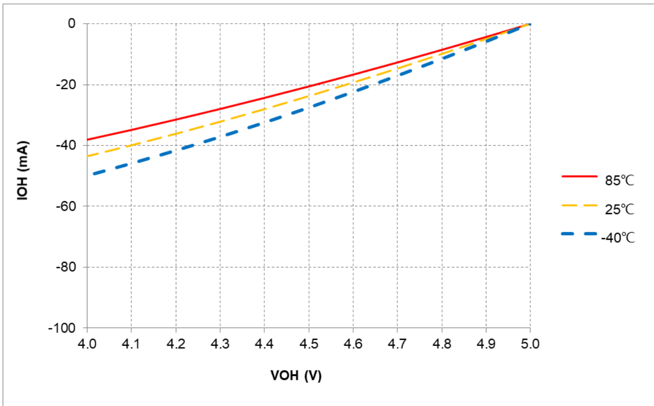
Figure 17-8 IOH vs. VOH @L3 = -24mA , VDD = 5V
