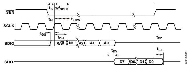
Figure 48. SPI 4-Wire Read Operation Timing
