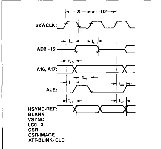
Display Memory Display Cycle Timing
