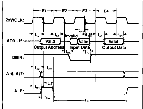
Display Memory RMW Timing
