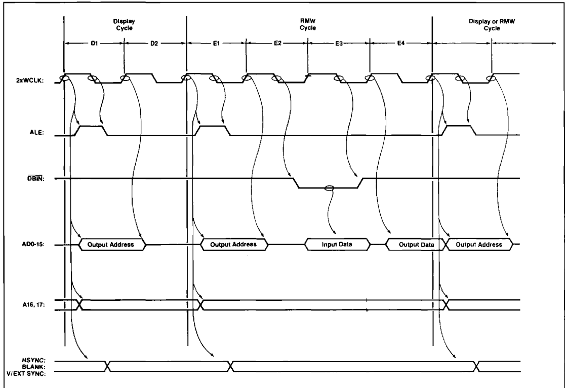
Display and RMW Cycles (1x Zoom)
