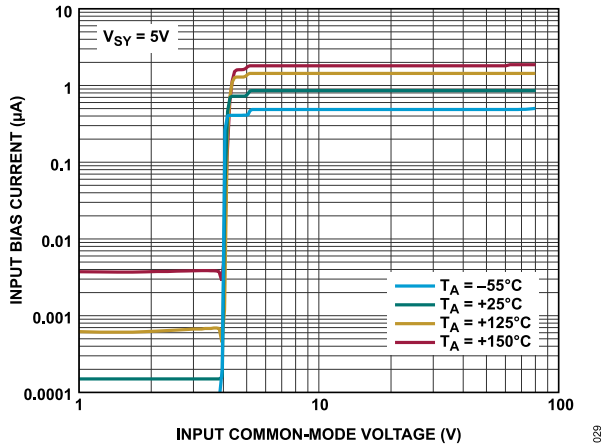
Figure 31. Input Bias Current vs. Input Common-Mode Voltage
