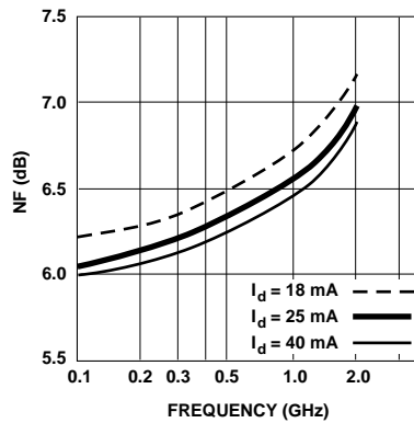
Figure 5. Noise Figure vs. Frequency.
