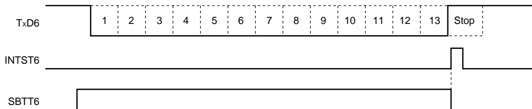
Figure 14-23. SBF Transmission
