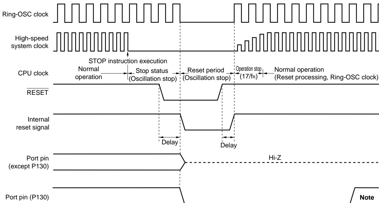
Figure 19-4. Timing of Reset in STOP Mode by RESET Input
