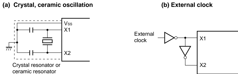
Figure 5-9. Examples of External Circuit of High-Speed System Clock Oscillator
