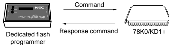
Figure 24-16. Communication Commands
