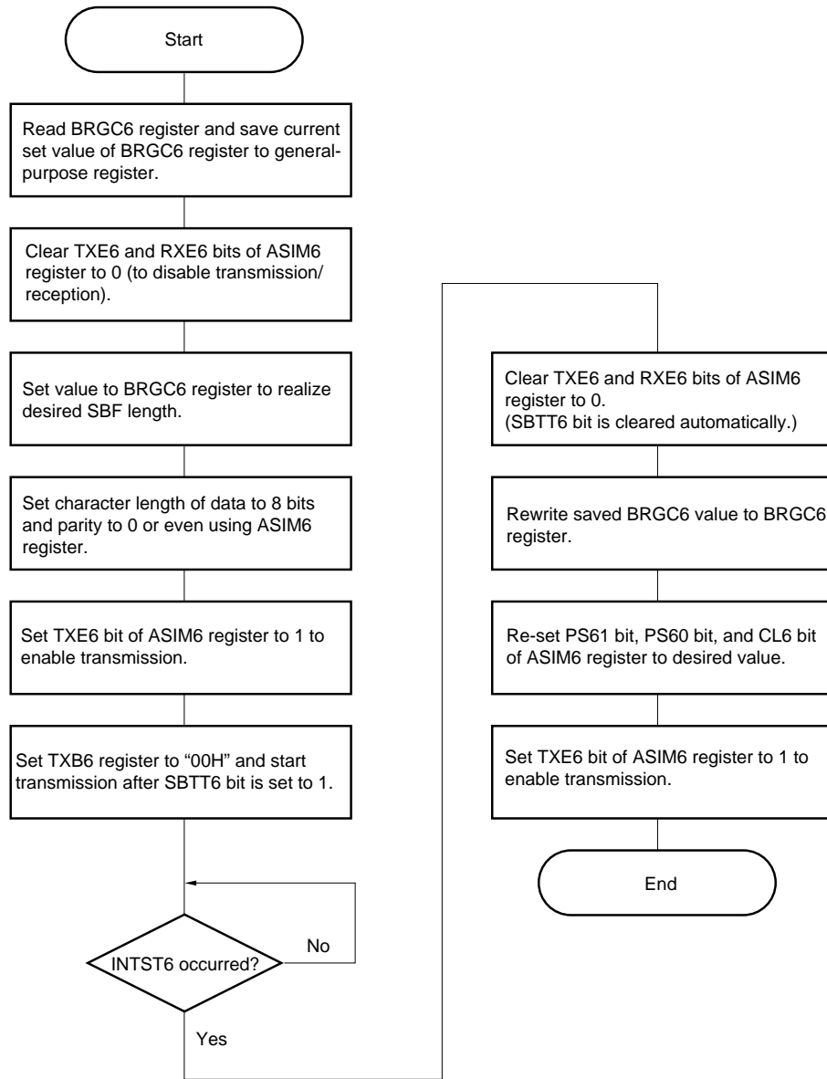
Figure 14-23. SBF Transmission
