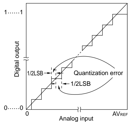
Figure 12-14. Quantization Error
