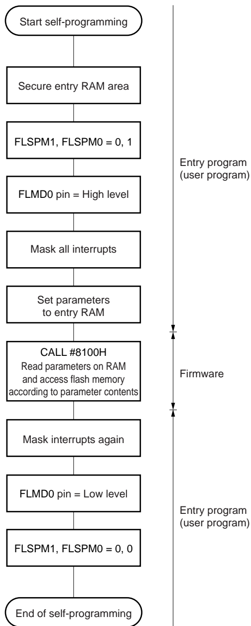
Figure 24-17. Self-Programming Procedure
