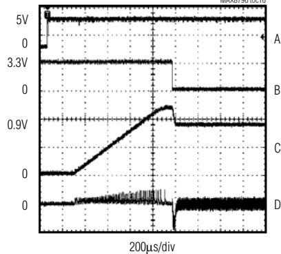
MAX8796/MAX17401 IMVP-6 SOFT-START WAVEFORM (UP TO CLKEN)
