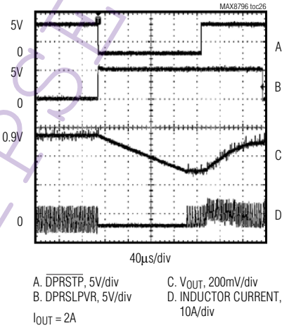
ENTERING DEEPER SLEEP EXITING TO LFM
