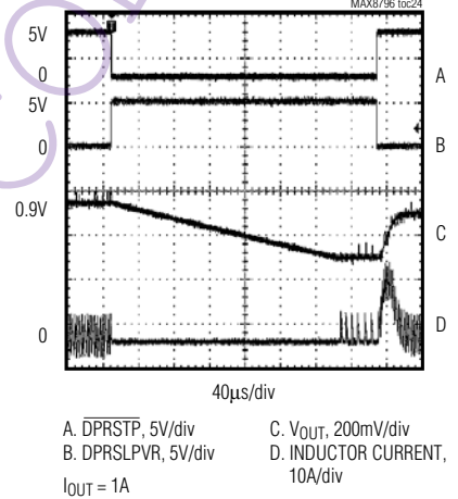
ENTERING DEEPER SLEEP EXITING TO LFM
