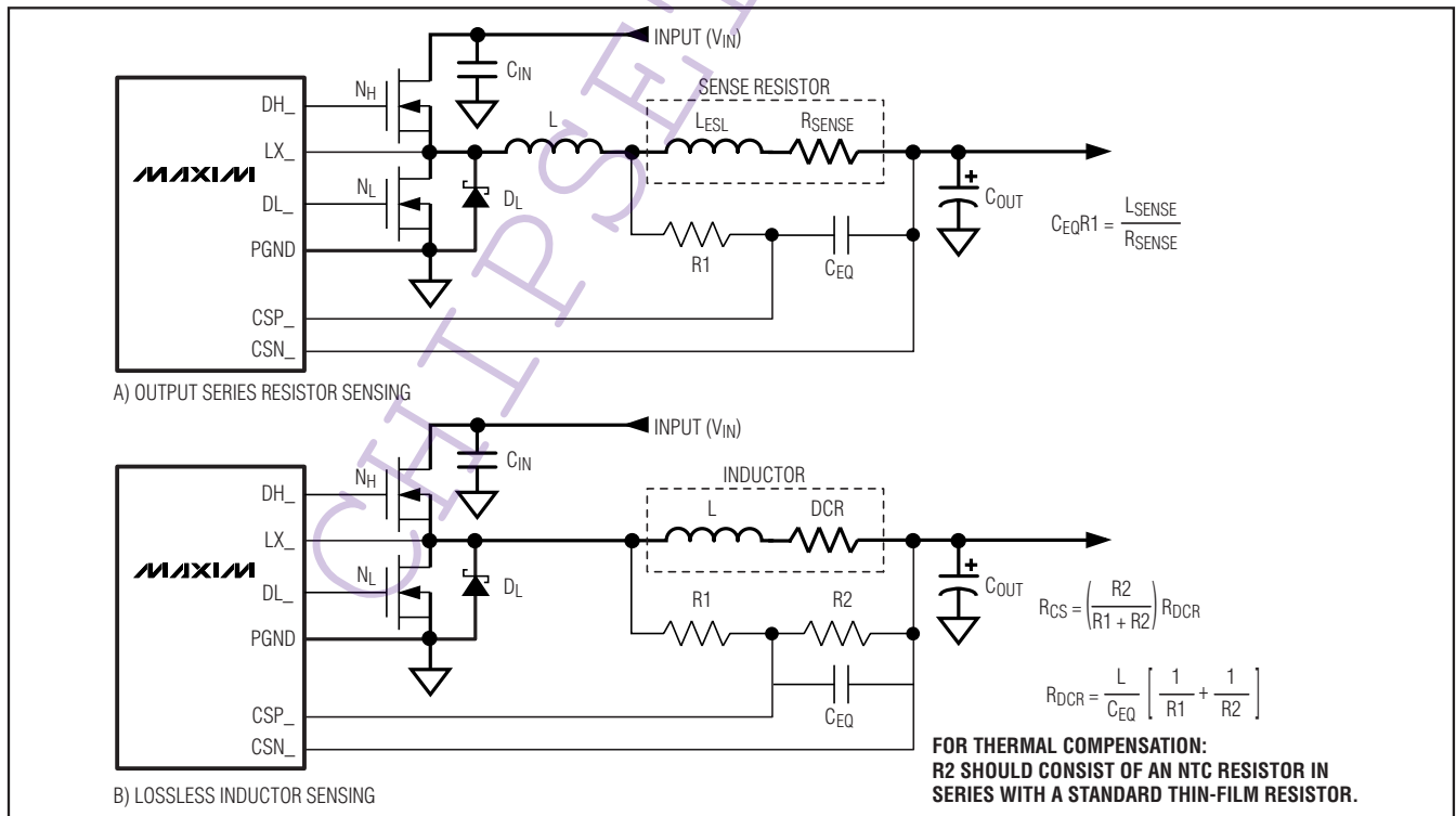
Figure 4. Current-Sense Methods
