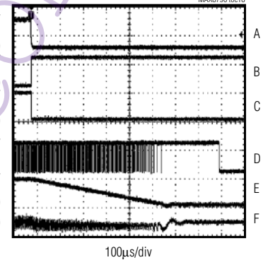
MAX8796/MAX17401 IMVP-6 SHUTDOWN WAVEFORM
