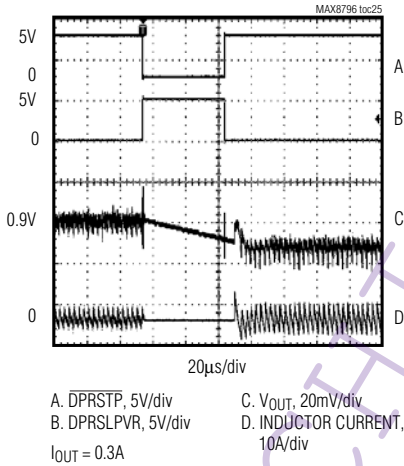
ENTERING DEEPER SLEEP EXITING TO NEAREST VID
