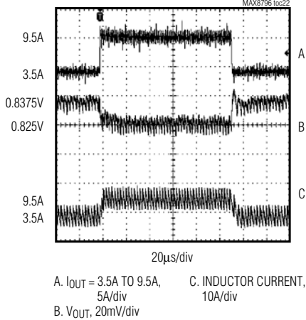
MAX8796/MAX17401 LOAD-TRANSIENT RESPONSE (IMVP-6 LFM MODE)
